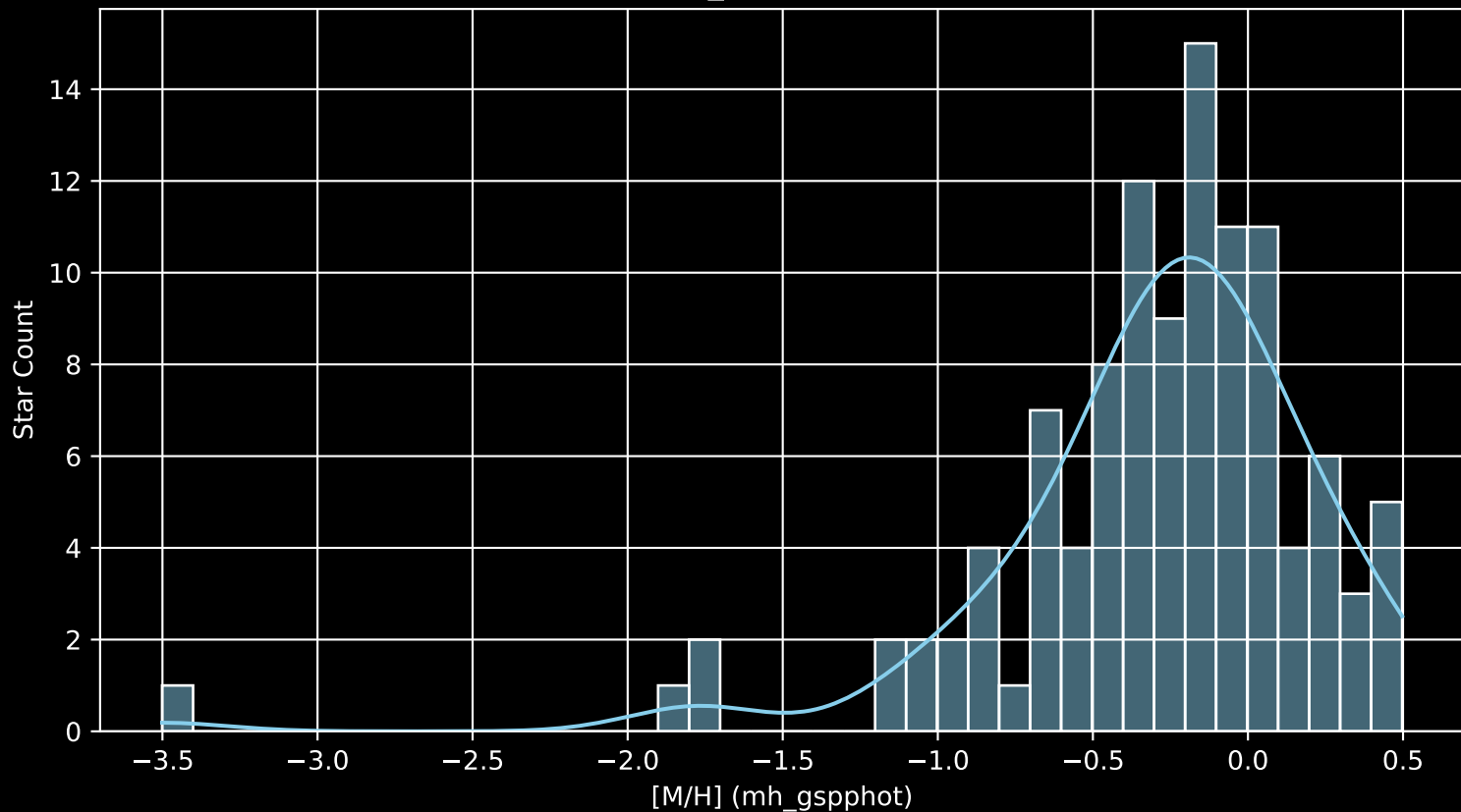
APOGEE DR17 Field: [280-32-O_TESS [M/H] (mh_gspphot) (n= 110)
