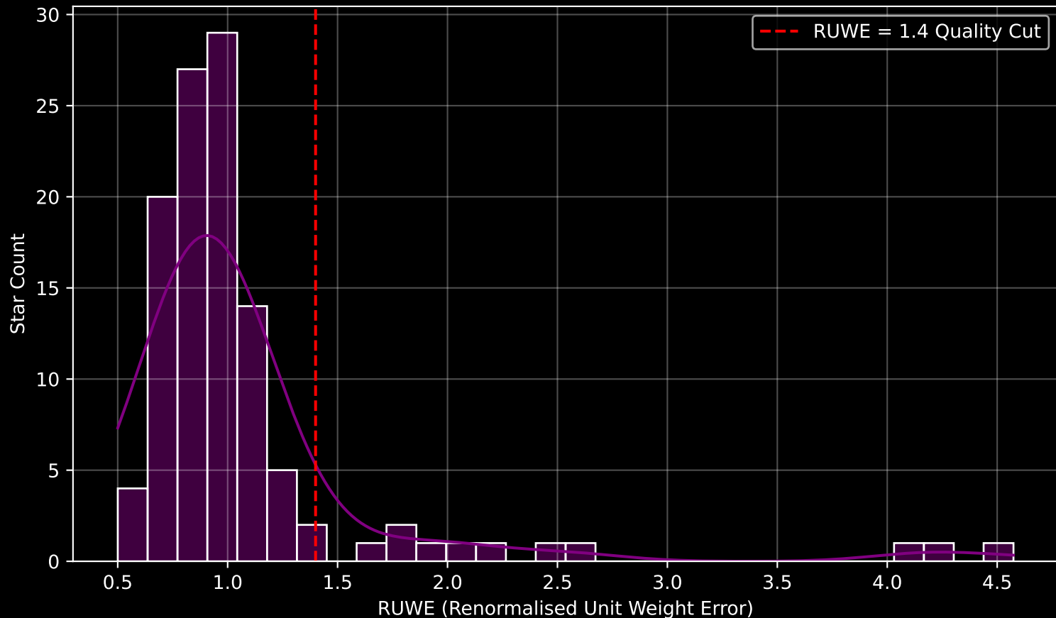
GAPOGEE DR17 Field [280-32-O_TESS] RUWE Distribution (n= 112)
