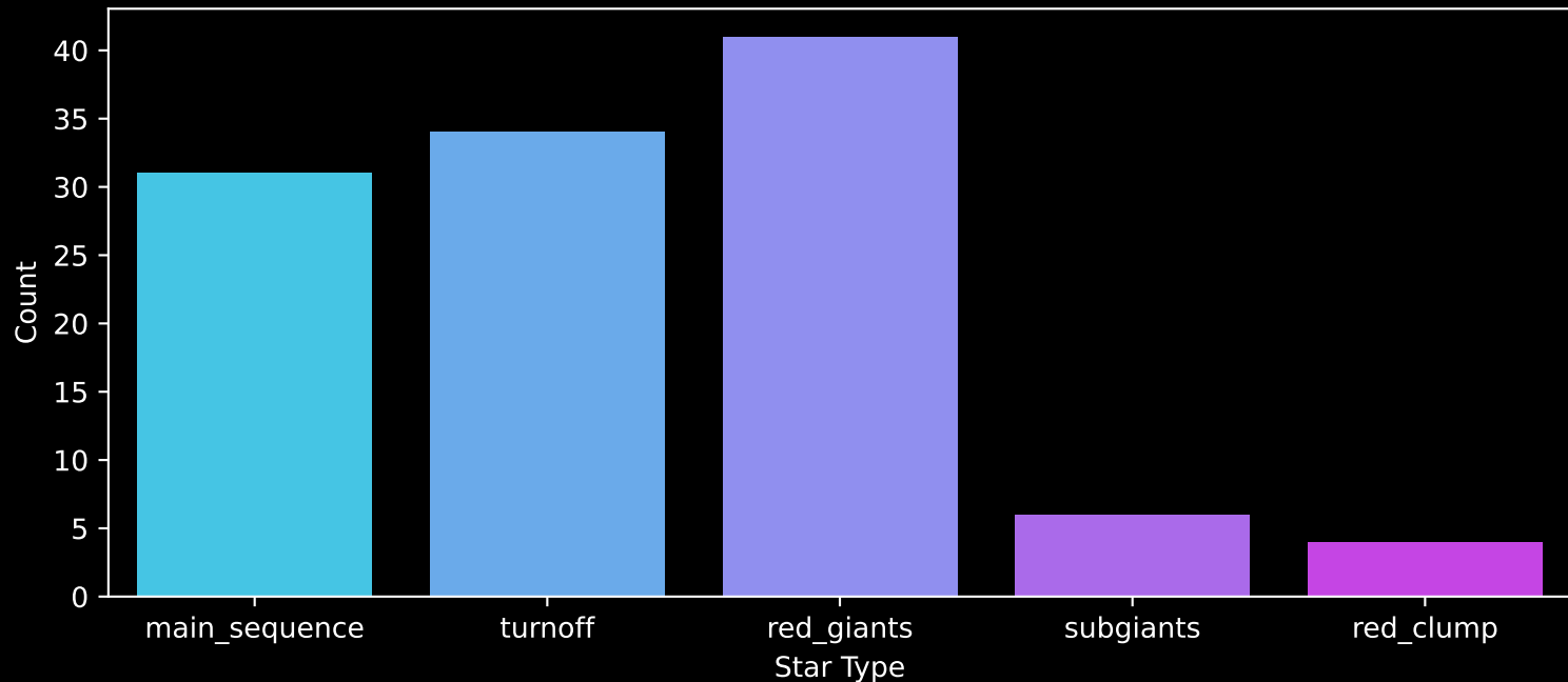
APOGEE DR17 Field: [280-32-O_TESS] Count plot of Star Type
