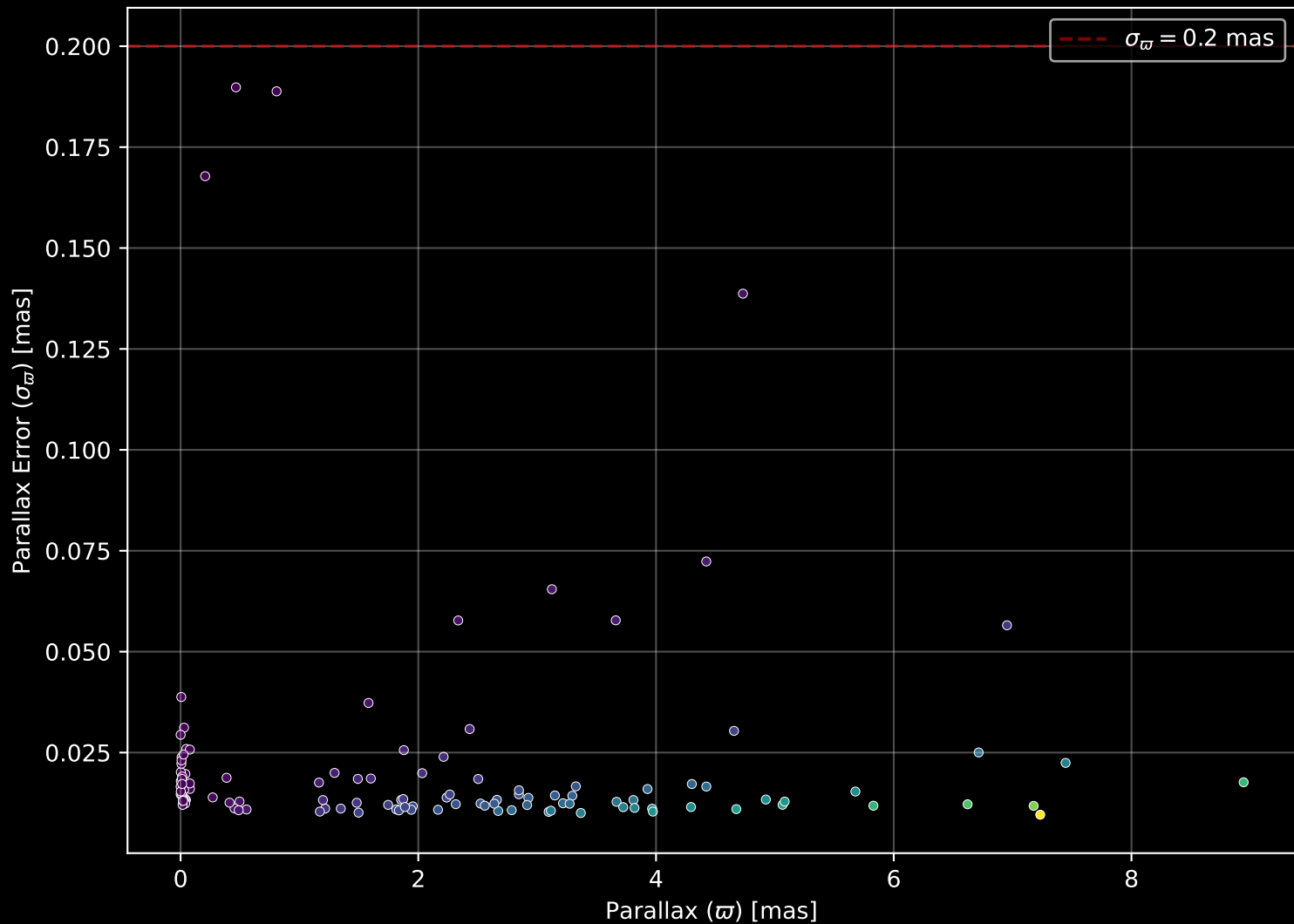
APOGEE DR17 Field: [280-32-O_TESS] Parallax Quality (n= 116)
