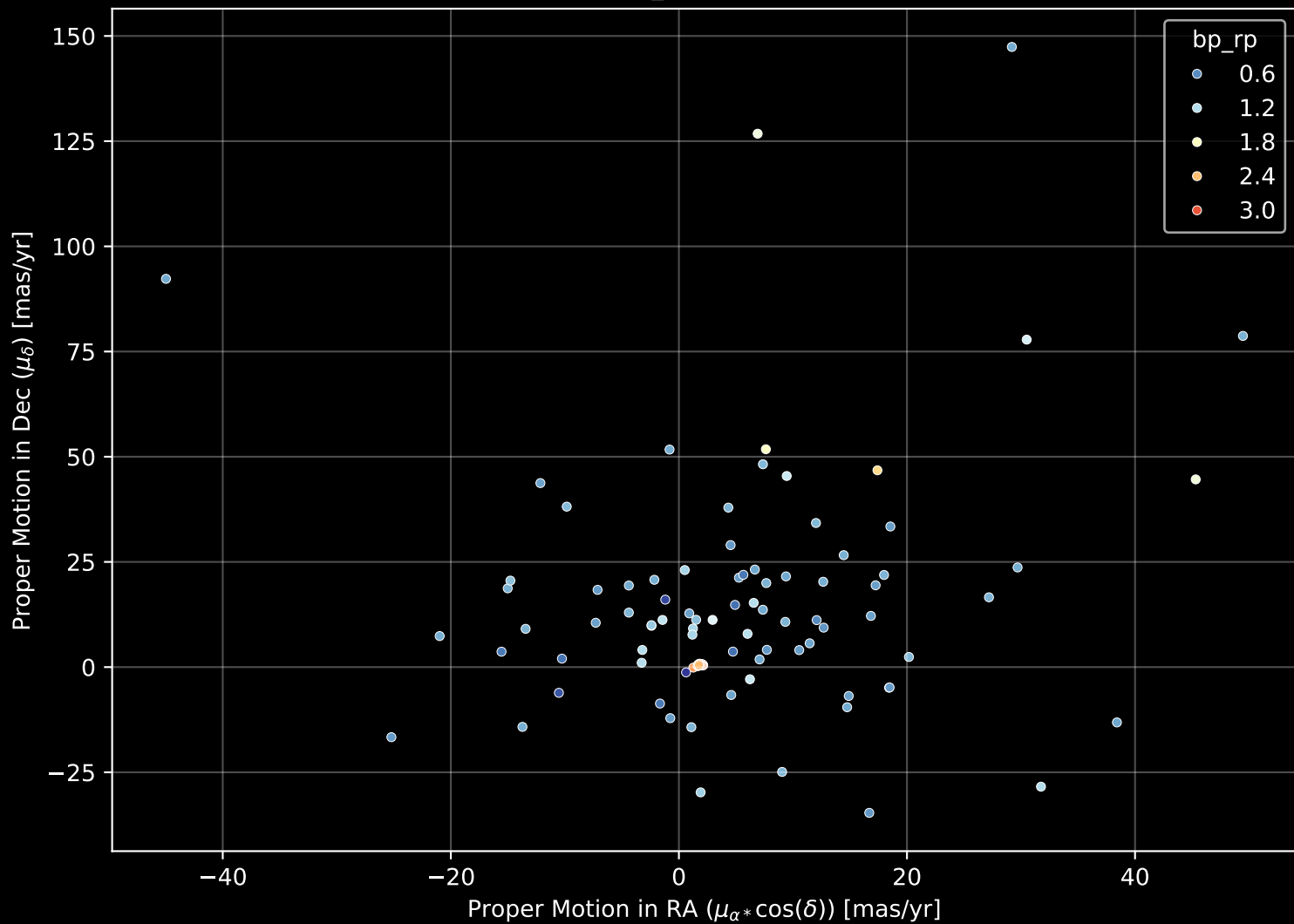
APOGEE DR17 Field: [280-32-O_TESS] Proper Motion Diagram (n= 116)
